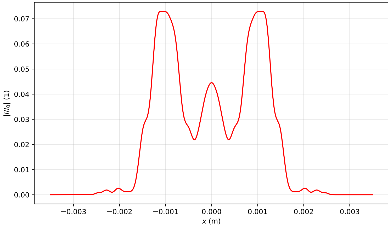
Intensity profile I(x, y = 0, z = 2.866)/I_0 , P_{in}=6.5P_{cr} , artificial time
